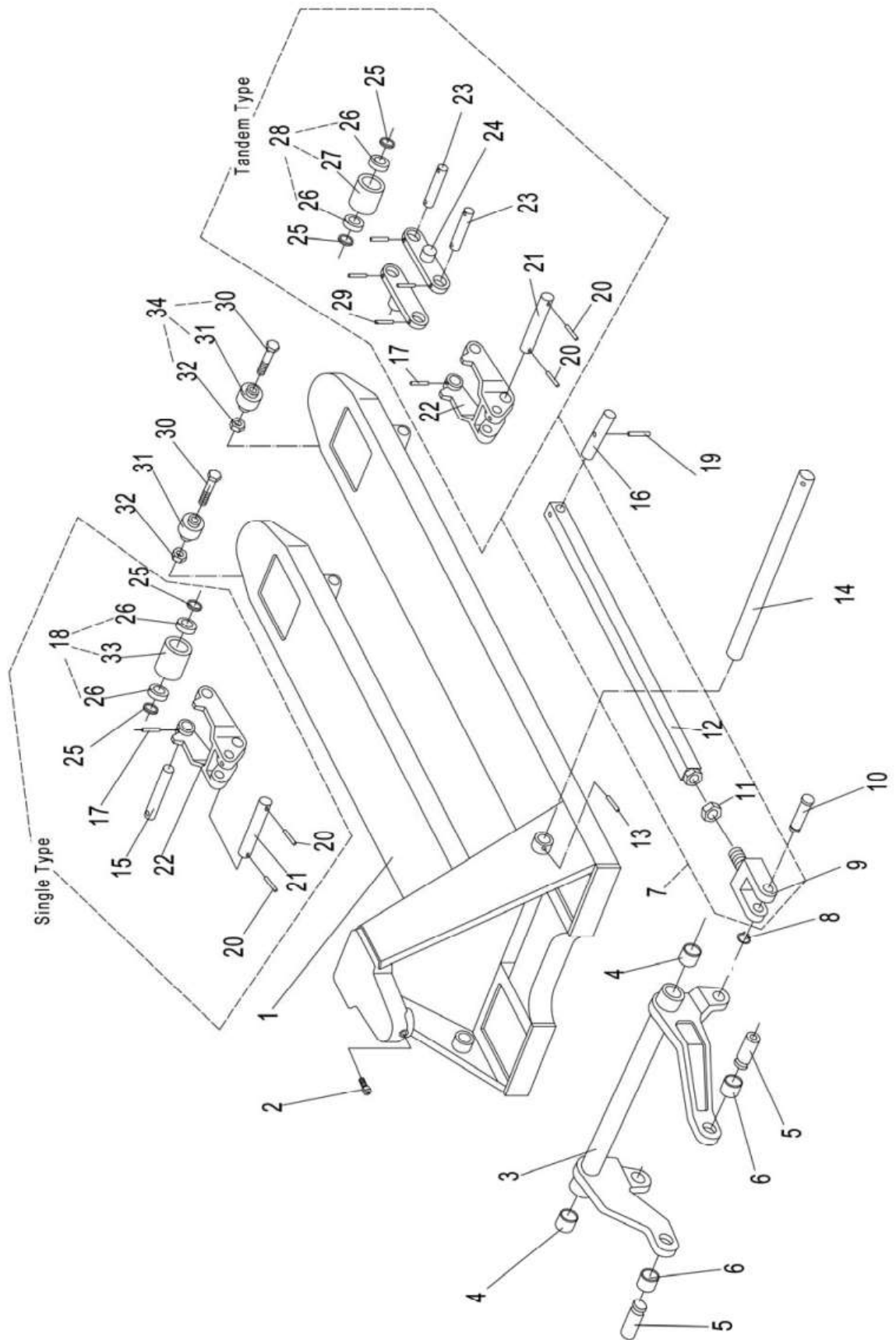
Fig.2 Fork Frame
